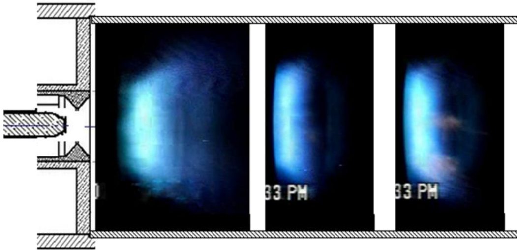
Figure 90. Flame in the combustor at (a) P=1\text{atm} , T=663\text{K} , V=14 m/s, \Phi_{\text{overall}}=0.41 (b) P=2\text{atm} , T=682\text{K} , V=10.6\text{m/s} , \Phi_{\text{overall}}=0.28 (c) P=4\text{atm} , T=733\text{K} , V=12\text{m/s} , \Phi_{\text{overall}}=0.23 .
