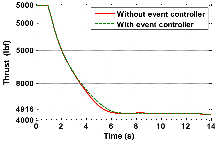
Figure 82. Thrust responses for the modified RU limiter case and with event based control case.
