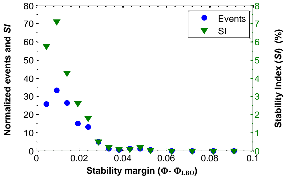
Figure 43. Average event rate and Stability Index ( SI ) for instability w/o \Phi' obtained from low-pass filtered optical signals. Left vertical axis scale: event rate and SI normalized with average event rate SI in the range \Phi - \Phi_{\text{LBO}} = 0.03-0.05 . Right axis scale: actual scale for SI .
