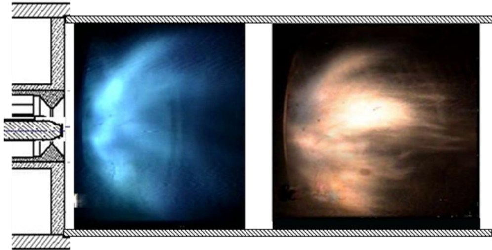
Figure 88. Flame in the LDI combustor for (a) P=1.17 atm, T=663 K, V=14 m/s, \Phi_{\text{overall}}=0.5 (b) P=2 atm, T=682 K, V=10.6 m/s, \Phi_{\text{overall}}=0.3 .
