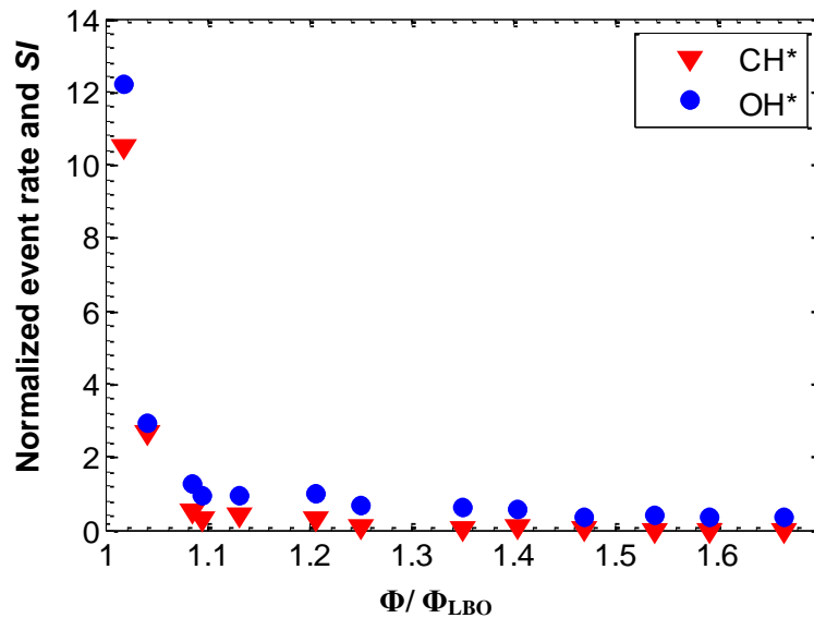
Figure 55. Average event rate from low-pass filtered \text{CH}^* and \text{OH}^* signals with same threshold settings.
