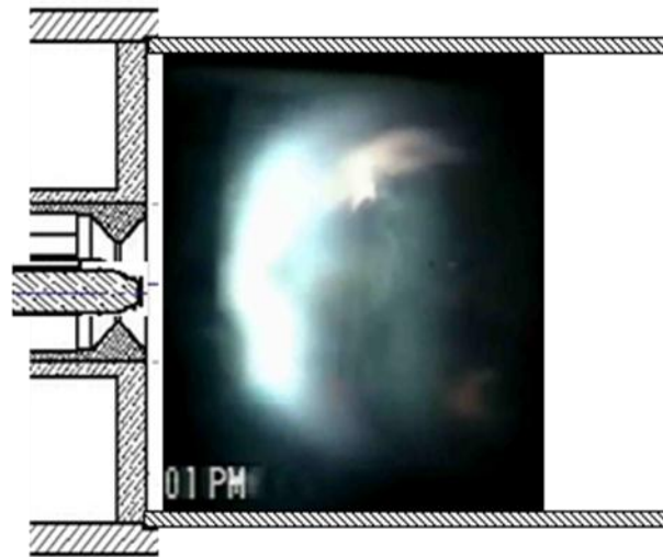
Figure 89. Flame in the combustor at P=1.13 atm, T=654 K, V= 13.4 m/s, \Phi_{\text{overall}}=0.32 , for fuel nozzle position upstream of venturi throat.
