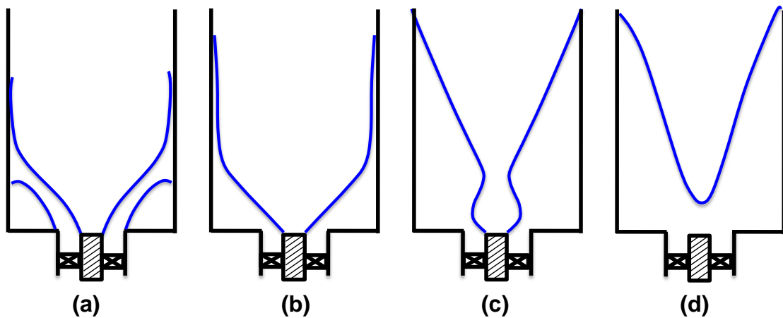
Figure 5. Illustrative flame configurations in premixed swirl combustors.
